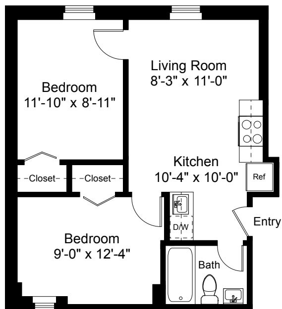
Unit 4 Floor Plan
