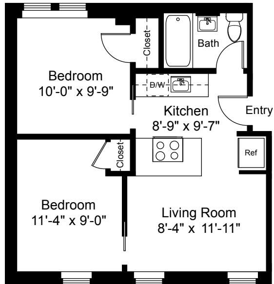
Unit 5 Floor Plan
